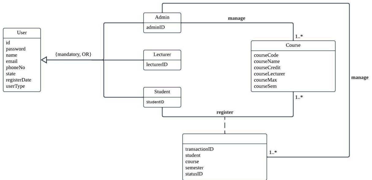
Figure 2.2.1 Conceptual Entity Relationship Diagram for Course Registration System
