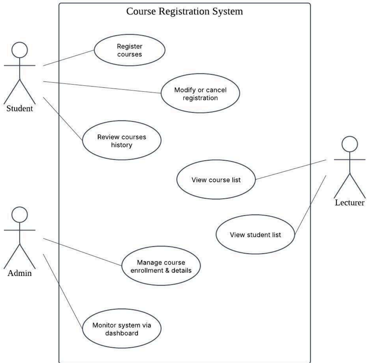
Figure 2.1.1 Use Case Diagram for Course Registration System
