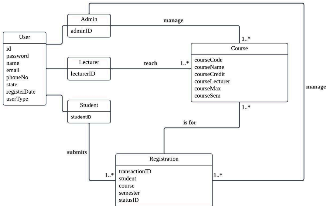
Figure 2.2.2 Logical Entity Relationship Diagram for Course Registration System
