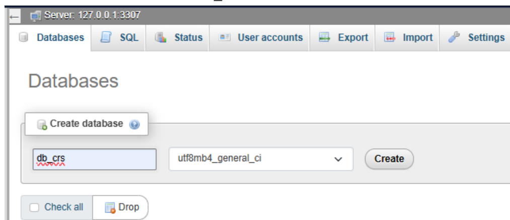
Figure 7.0.3 Create Database
