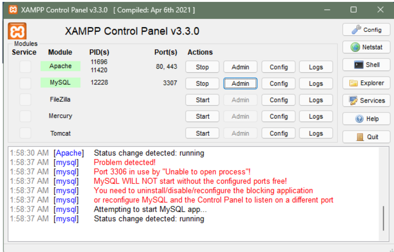
Figure 7.0.1 XAMPP Control Panel
