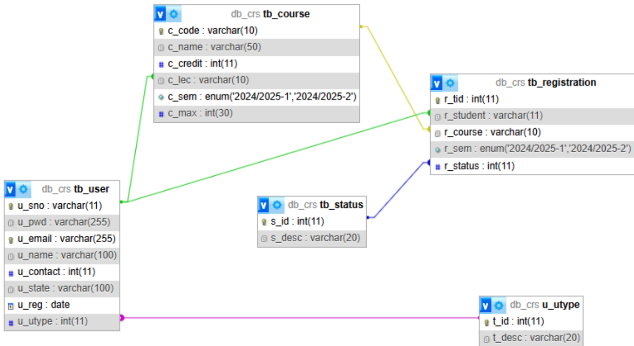
Figure 4.0.1 Designer Diagram for Course Registration System
